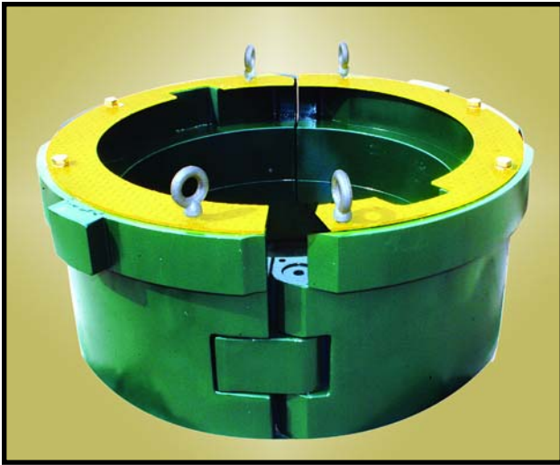
Frank's 49 1/2" x 37 1/2" Hinged Adapter Bushing
